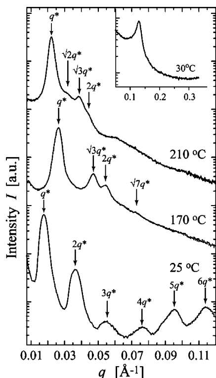
Figure 6. SAXS intensity patterns for PS- block -P4VP(MSA) 1.0 (PDP) 1.0 with the f_{\text{comb},2} = 0.40 (sample S40.67k.MP). The curves have been measured upon heating 5^\circ\text{C}/\text{min} and show characteristic reflections for LAM, CYL', and SPH' structures. The SAXS curve corresponding to the smaller length scale structure within supramolecular comblike P4VP(MSA) 1.0 (PDP) 1.0 at T = 30^\circ\text{C} is shown in the inset, whereas at T = 170^\circ\text{C} and T = 210^\circ\text{C} no distinct reflections are observed due to ODT.
